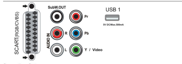
Connections Bottom
